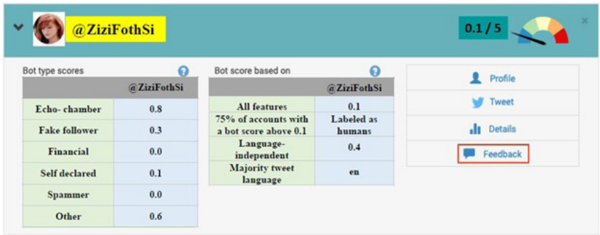
Figure 3. Botometer results
