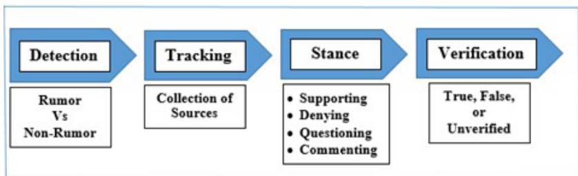
Figure 1. PHEME process
